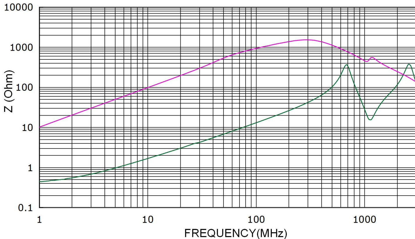
CHOK4532S801A10T
