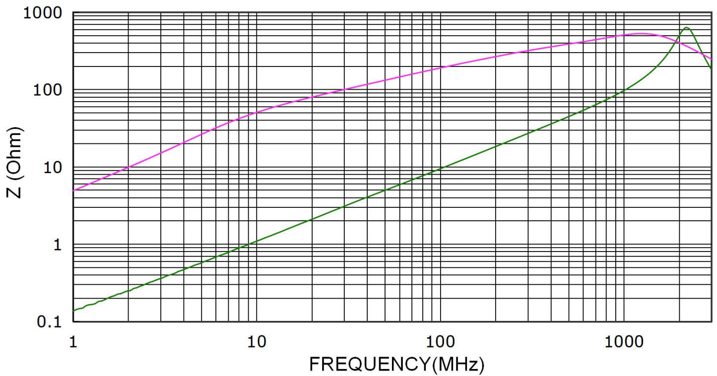
CHOK4532S231A35T
