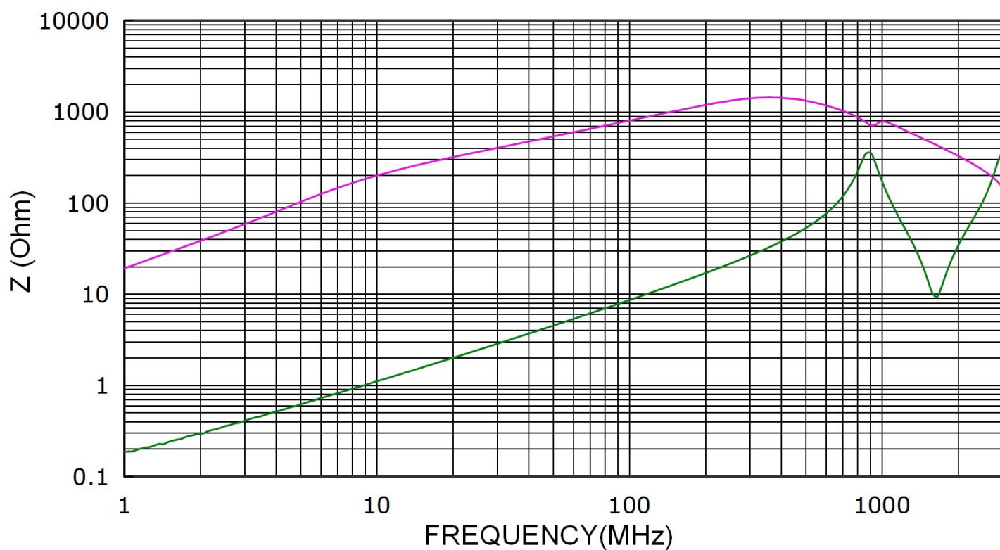
CHOK4532S901A23T
