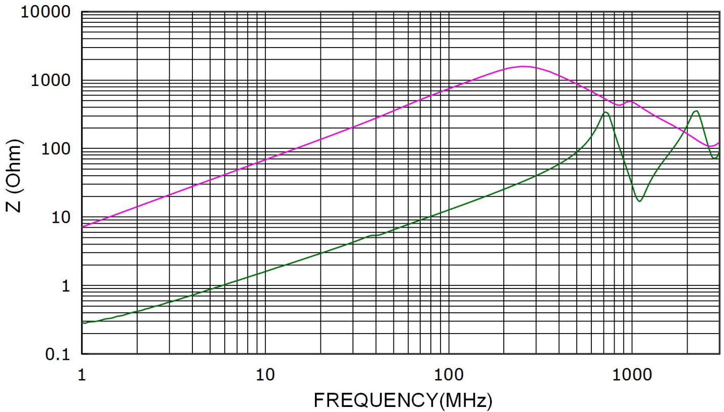
CHOK4532S601A15T
