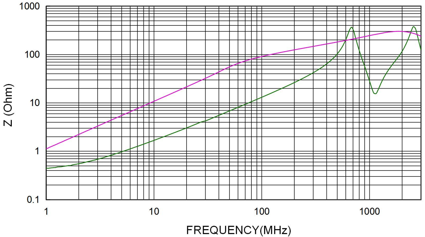
CHOK4532S121A30T
