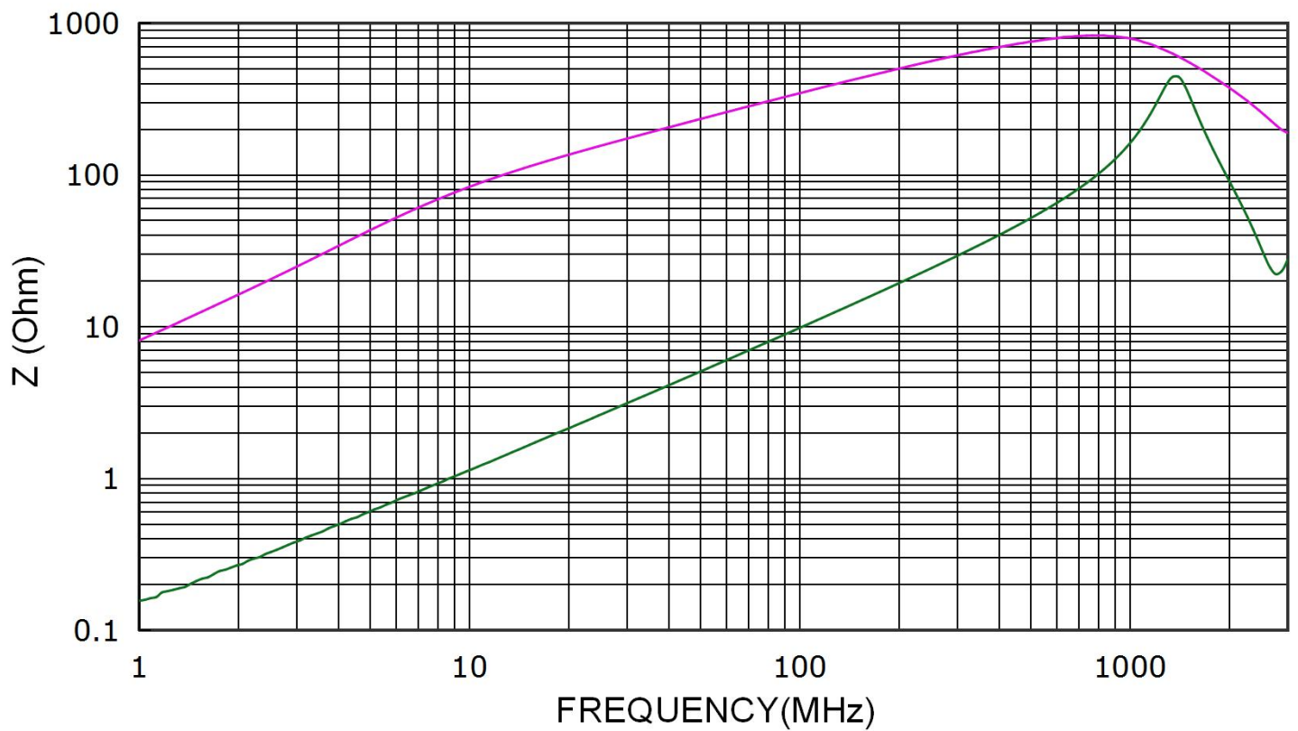
CHOK4532S421A32T
