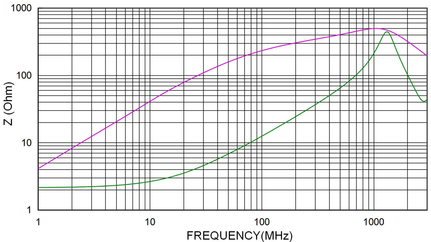
CHOK4532S201A15T
