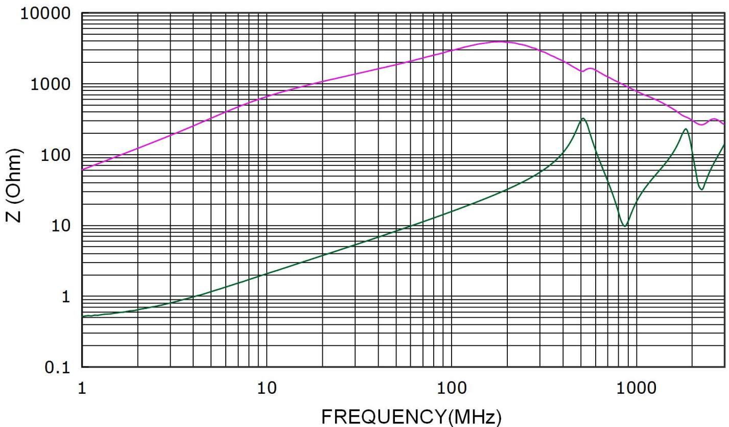
CHOK4532S282A09T
