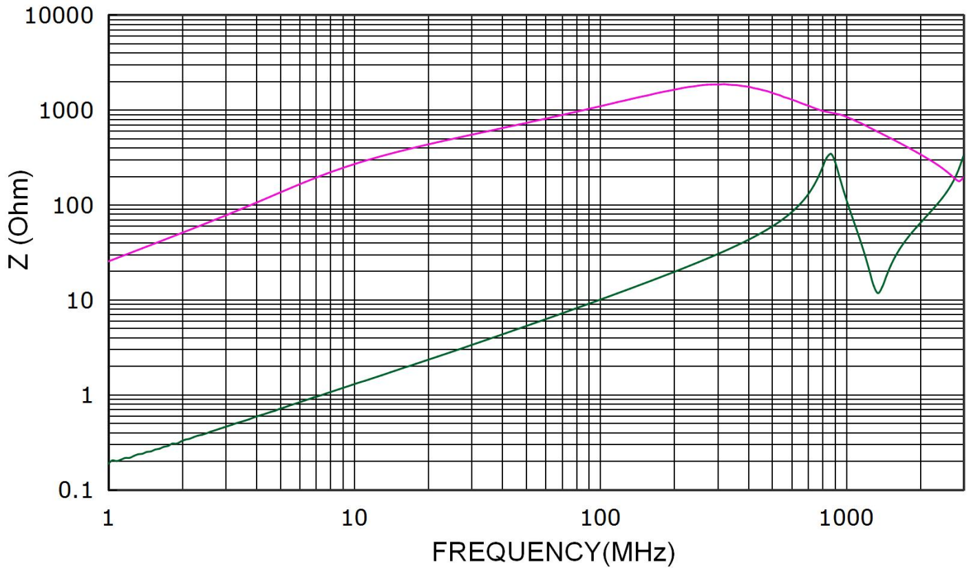
CHOK4532S142A20T
